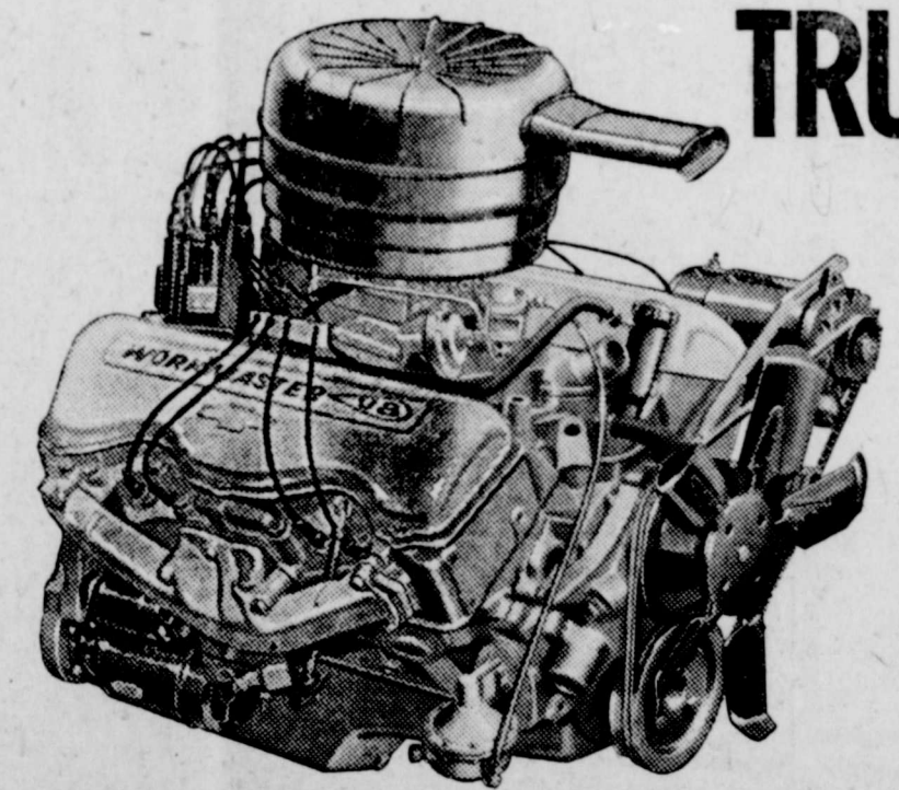
New Workmaster V8 featured in Spartan Series 90 and 100 heavy-duty models.
