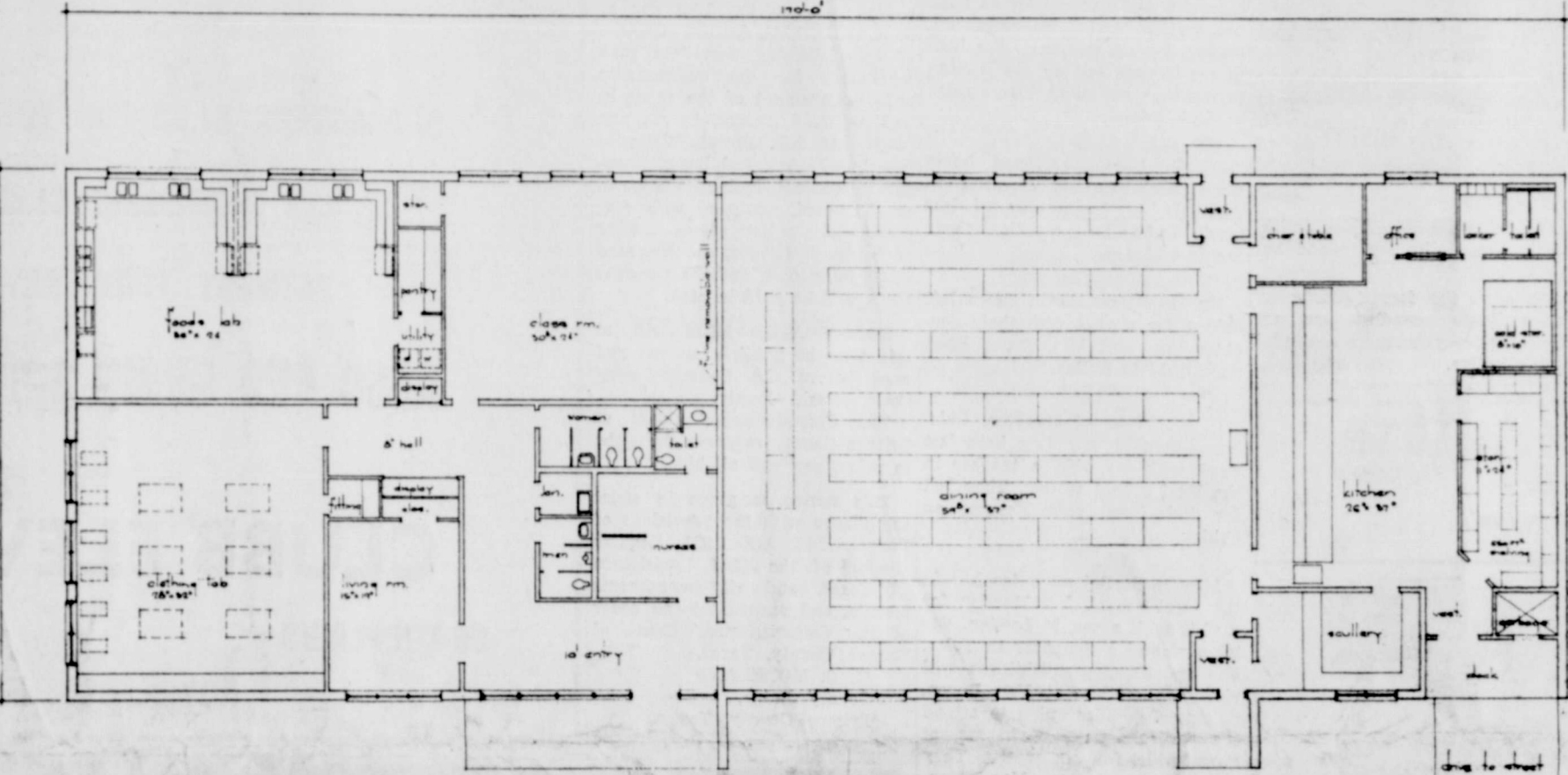
Floor plan of the proposed new homemaking department, nurse's office, film projection room, cafeteria, and kitchen for the Silverton Independent School District. Additional primary classroom and janitor's work room to be constructed adjoining west end of existing primary wing. (Drawing by Bill Cox of Lubbock.)
