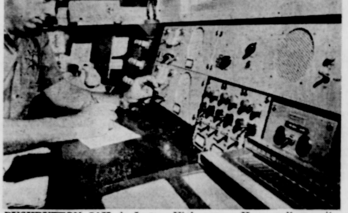
PUSHBUTTON JAIL in Logan, Utah uses a Honeywell security console to electronically keep the prisoners locked up safely in their cells. One man can control whole jail from this unit.
