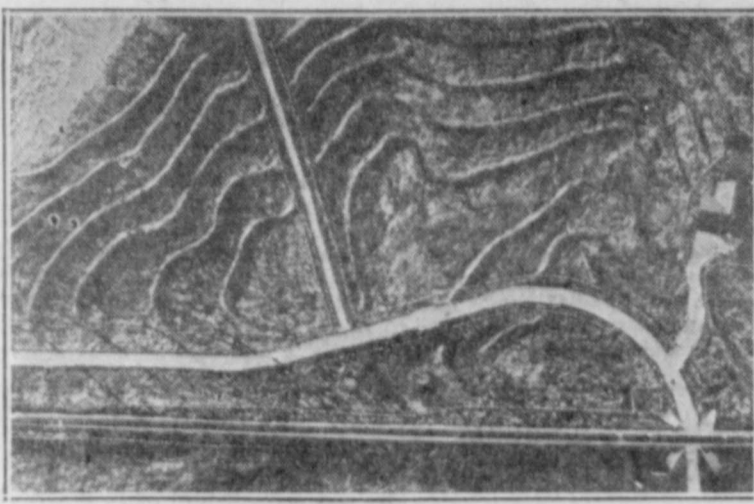
This view is of a clay model of the terracing demonstration four miles west of Abilene on Highway 1. The entire drainage area is terraced with level terraces joined to highway, county road, private drive ways, and railroad embankment, eliminating soil erosion and conserving all the water falling in the area. The project stopped flow of water through five bridges.
