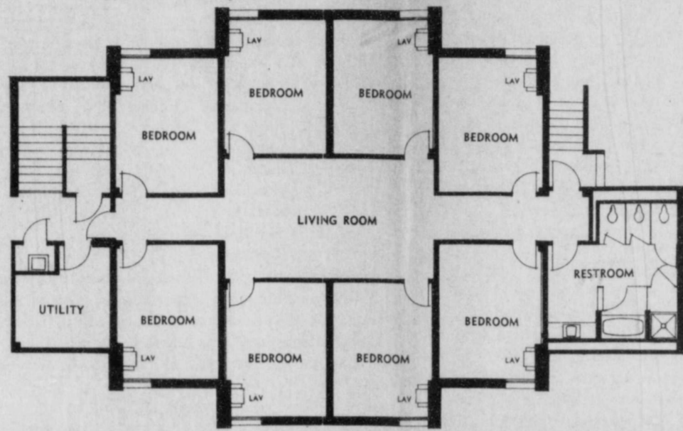
Typical Dormitory Pod
