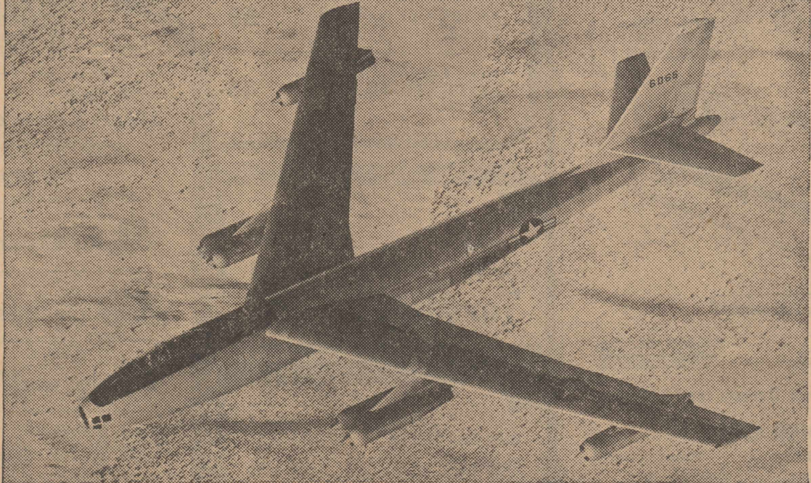
BOEING B-47 STRATOJET, holder of the transcontinental record of 3 hours, 46 minutes at an average speed of 607.8 miles per hour. Comparable in size to the famed Boeing B-29 Superfortress, the B-47 has six jet engines under its swept-back wings. Eighteen Jato rockets are carried in the sides of the fuselage for use in emergency or heavy-load takeoffs. The U.S. Air Force has ordered the Stratojet into production at the Wichita plants of the Boeing Airplane Company.
