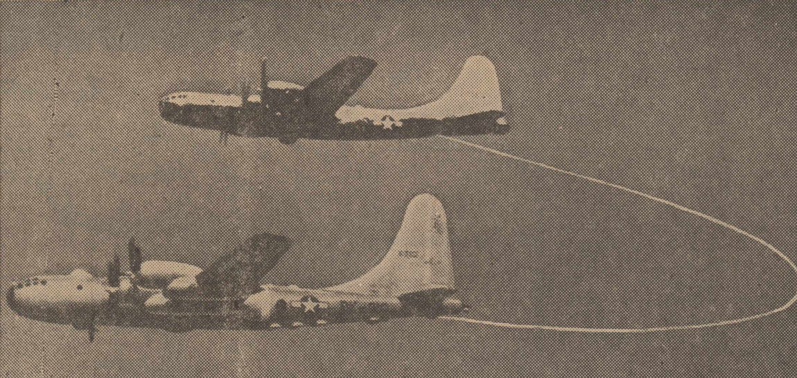
HERE'S HOW AIR REFUELING JOB WAS DONE . . . This photo of refueling of the Lucky Lady II, which flew non-stop around the world in 94 hours, shows how the B-50 was supplied with fuel for the 23,452 miles. The bomber was refueled in this fashion at four points on the flight—the Azores, Saudi Arabia, the Philippine Islands and the Hawaiian Islands. The refueling technique was worked out especially for the flight. A top officer of the air corps declared that the flight had definitely established the fact that the United States was now in position to deliver the atom bomb "wherever it might be required." When that might be remained an unknown quantity.
