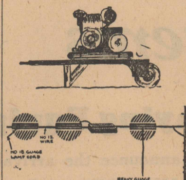
Shown in the top drawing is the generator used in powering the electric seine, and, below, details of the seine's construction.
