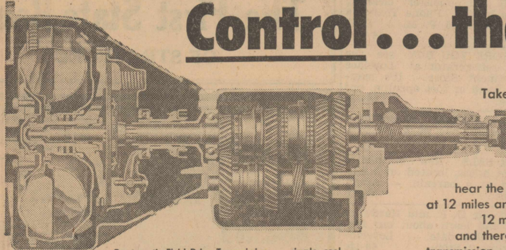
Prestomatic Fluid Drive Transmission... simple, cool-running, with three rugged compact units designed with a minimum of moving parts... gyrul Fluid Drive, the Safety Clutch, and Prestomatic Transmission. Ruggedly built for trouble-free service.
