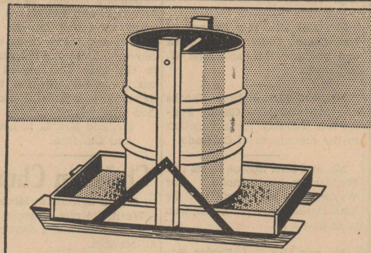
PORTABLE HOG FEEDER . . . Container is 50 gallon oil drum with both ends cut out. Flat bottom box is mounted on 4" x 4" pieces for skid runners. Upright braces on either side support pipe passed through uprights and barrel. Barrel swings half inch above bottom of box.
