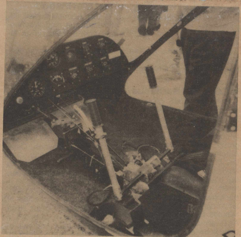
Shown is the inside of a gyrocopter's two-seater and instrument panel.
