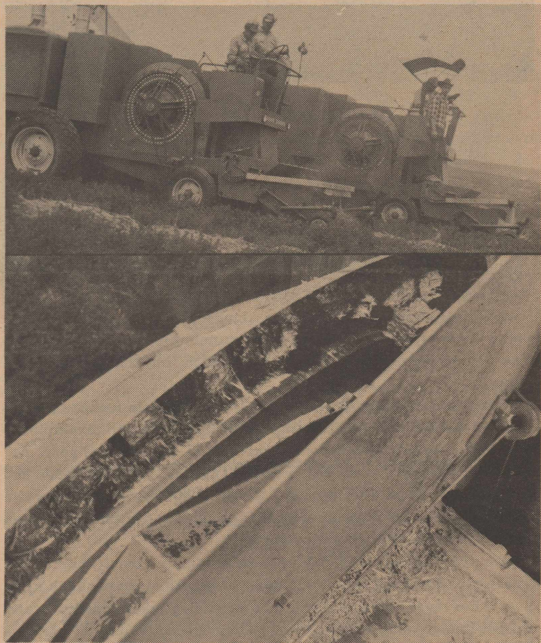
The 66 dies in this huge press wheel that produce the cubed alfalfa cost $2500 per set. (Thank goodness they last a long time.) The upper picture shows the die wheel as the machines are going down the field. The lower picture shows the cubes as they push out of the dies and fall into the elevator that transfers them to the truck on the Paul Conditt and Jim Paul farm.
