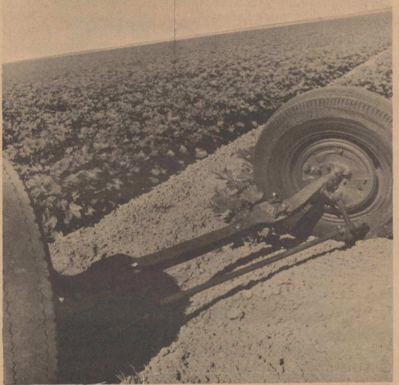
The bolts can be seen on the axle where they were sheared off and carried 300 feet down the highway. Final resting place - cotton patch.
