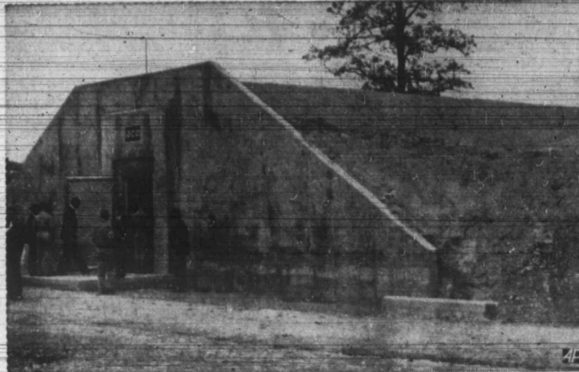
MAGAZINE NOT FOR READING—New type "Igloo" powder magazines such as this one in a southwest Virginia hillside are to be used to house the output of new gunpowder plants at Radford and New River, Va. The structures are of monolithic arch concrete construction, earth-covered and camouflaged to prevent aerial detection. They're also lightning-proof.
