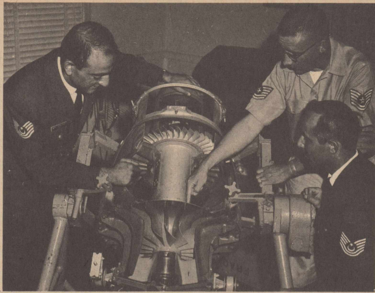
CLASSROOM — Jet engine repair instructor, TSgt. James T. Croxson, explains details of a cutaway model of the J69-T-25 engine used on the T-37 jet trainer to two members of the Turkish Air Force undergoing training at Reese. The two students are Master Sergeants Ihsan Pinar, left, and Sukru Erten, right.
