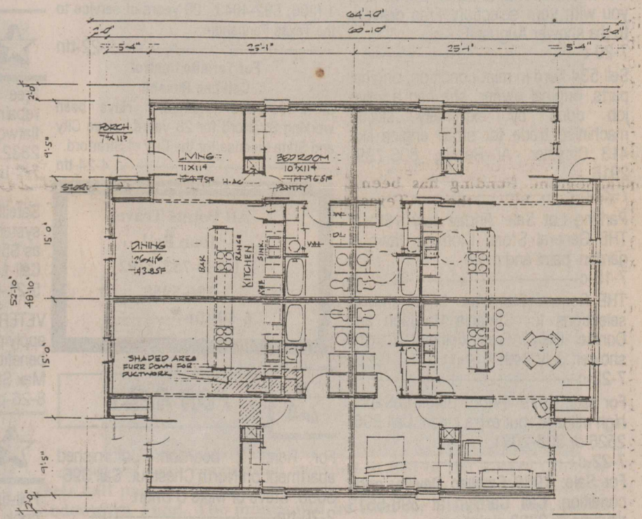
FLOOR PLAN TYPICAL FOURPLEX Scale: 1/8"=1'-0"
