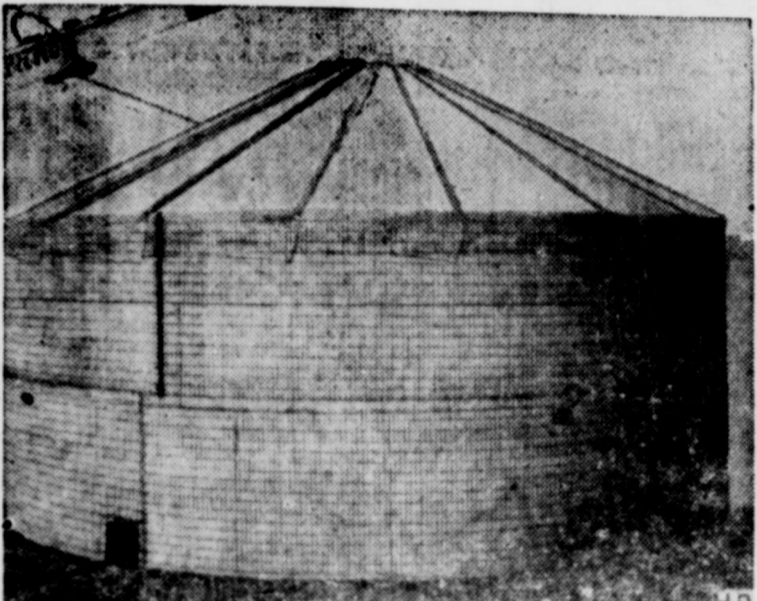
This grain bin, made of asphalt roll roofing and welded wire fencing has a capacity of about 1,300 bushels. It can be constructed in about 30 man-hours of work.
