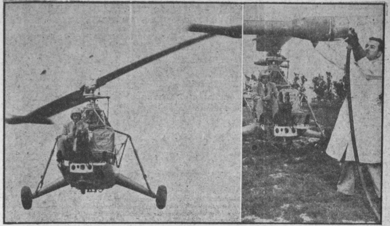
TEST NEW JET HELICOPTER —An experimental helicopter named the "Top Sergeant" takes to the air, left, at Manhattan Beach, Calif., powered by pulsejet engines mounted at the rotor tips. The pulsejet engines are unique in that they weigh a scant 25 pounds each, and contain only one moving part. At right, mechanic Charles Duschak squirts a spray of gasoline into the pulsejet mounted on the tip of a rotor blade, in preparation for a flight. Designing engineers say the new-type "flying windmill" will lift twice the payload of the conventional helicopter by eliminating the weight of a heavy piston engine, and should be produced at one-fourth normal cost.
