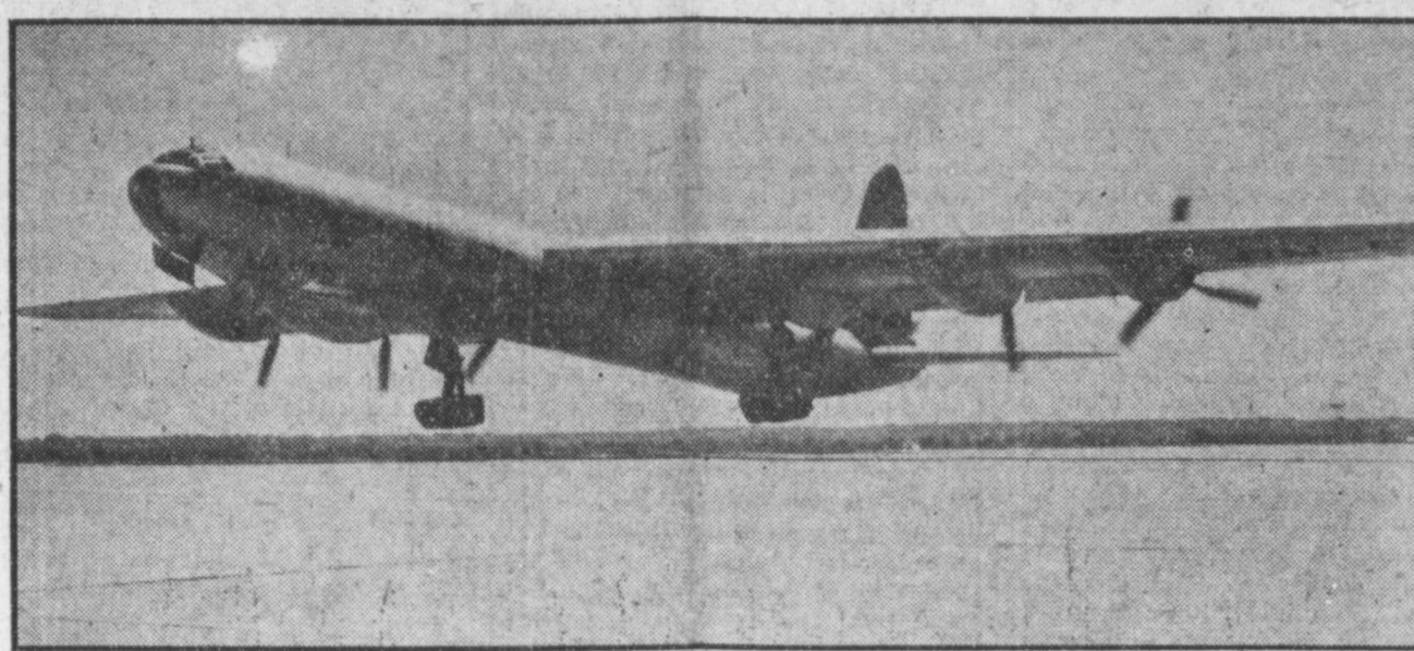
CATERPILLAR TREADS FOR SUPERBOMBER —The experimental XB-36 takes to the air at Fort Worth, Tex., equipped with the latest in landing gear—caterpillar-type track "wheels." The Air Force is making tests with this new device, in which the weight of the six-engine plane rests on bogie wheels rolling on two endless belts on each landing gear strut. Standard models of the B-36 bomber are equipped with four-wheel main landing gears and a dual nose wheel.
