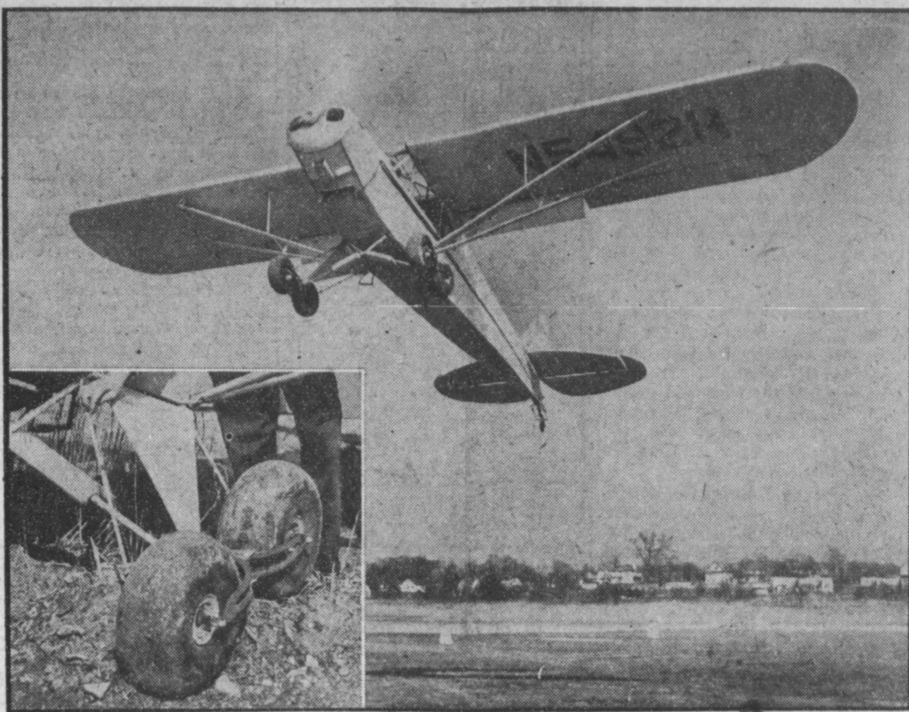
NEW CUB FEATURES SHORT RUN TAKE-OFF —After a take-off run of approximately five times its own length, the new Piper "103" Super Cub climbs into the air at Flushing Airport in New York. The versatile new lightplane, with a 108-horsepower engine, can maintain level flight at speeds as low as 30 m.p.h. in still air. Ideal for rough jobs such as crop dusting and spraying, some models of the craft are equipped with tandem landing gear (inset), making it possible to land on rough surfaces. The forward balloon tire carries only four pounds of air pressure, enabling it to climb small obstacles.
