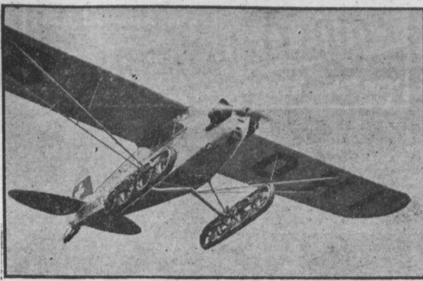
MAKING TRACKS —The first plane equipped with caterpillar tracks is pictured over airfield, near Rome, Italy, on test flight. Inventor Count Giovanni Bonmartini, who adapted the tracks to an airplane, claims the new landing gear allows the aircraft to land on any type of field, with or without landing facilities.
