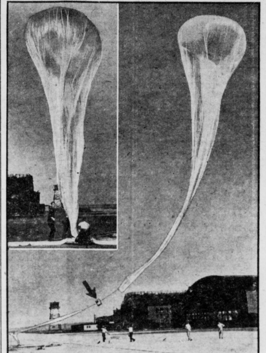
WATCH FOR 'EM! —Preparing to release one of many plastic balloons used for the Air Force project "Moby Dick" are launching crews who, naturally, think of this as a whale of an operation. The 50 to 110-foot diameter balloons are drifting over the United States at altitudes of 10 to 20 miles for the purpose of transmitting data concerning high-altitude winds. The transmitter (arrow) below the balloon sends out signals to direction-finding stations. Crew inflates one of the big bags (inset) which may appear as "flying saucers" during the early and late hours of the day because of sun reflections on the transparent coverings. Persons finding collapsed balloons will receive a reward for return of radio unit.
