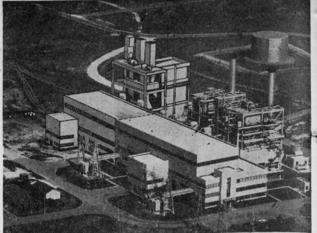
MORE POWER FOR SOUTH TEXAS—Here's how Central Power and Light Company's Lon C. Hill Power Station will look when a new 175,000-kilowatt generating unit is completed in 1959. Construction will begin this fall on the expansion which will more than double the size of the plant. The existing power plant is shown at the right, with an artist's sketch of the new addition at left.
