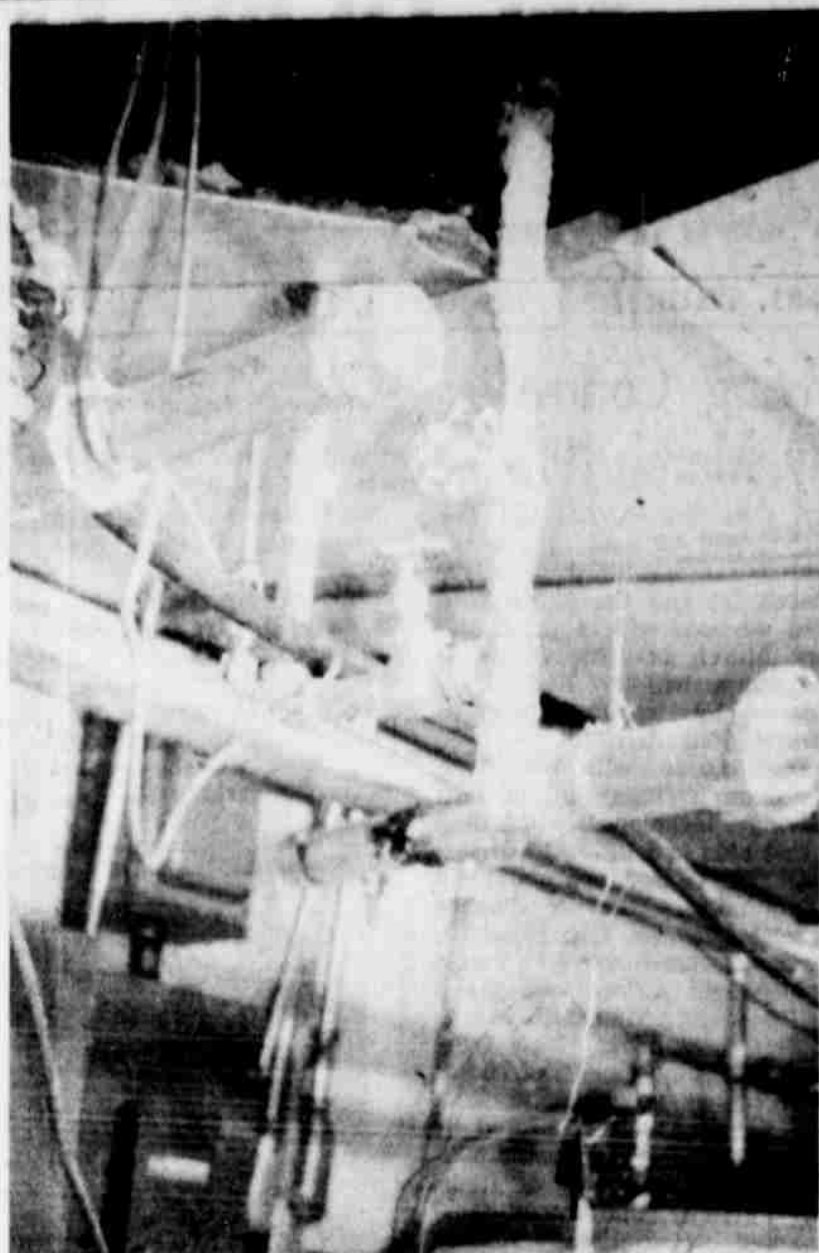
MORE PIPES TO THE STEAM HEAT BOILER that extend up into the ceiling of the basement show plainly the corrosion on pipes caused by Haskell's mineral-laden water. These pipes must be periodically scraped and replaced when necessary to maintain the heating system.
