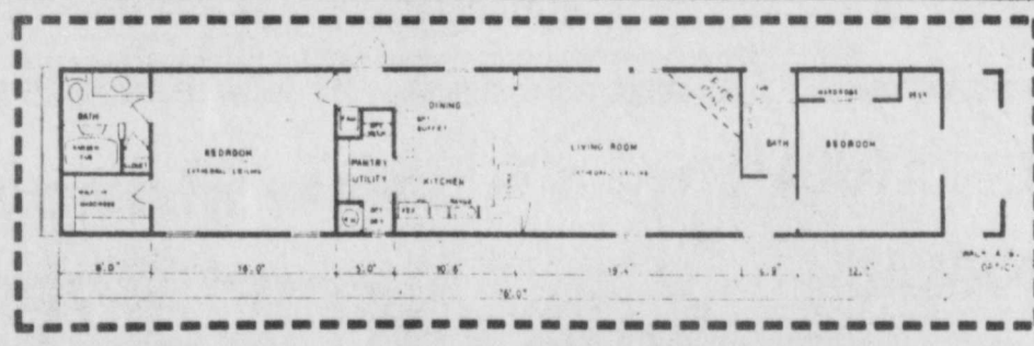
Peach Tree Model 1820 1064 Square Feet 14 x 80
