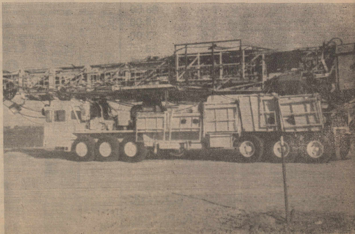
The drilling rig has arrived and is being readied to begin on the Tri-Ex Oil & Gas, Inc. 1-6 Exploration Unlimited W. H. Brooks (640 ac.) 467' from North and East line, Sec. 6, B-1, BS&F, eight miles east of Silverton. The permit is for drilling to 9000 feet. —Briscoe County News Photo
