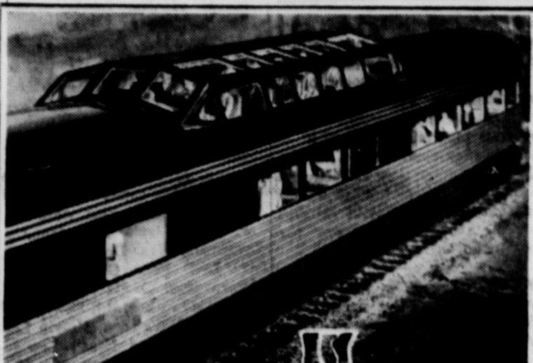
ASTRA DOME —This scale model of the observation lounge car of the General Motors Train of Tomorrow shows construction typical of the four Astra Dome coaches now nearing completion by Pullman-Standard Car Mfg. Co. This modernistic train, when completed, will tour leading cities.
