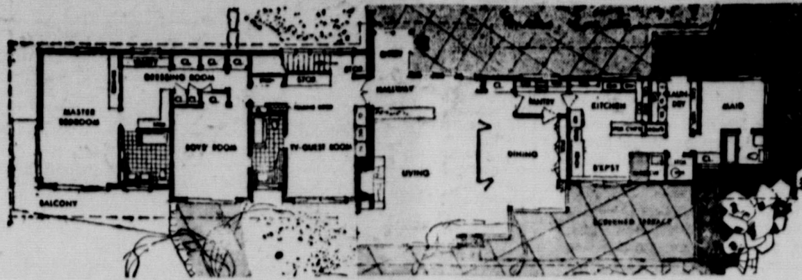
This is the floor plan for "The Pace Setter House of 1953," located at Bronville, New York. The subject of more than 60 pages of text and illustration in the November issue of House Beautiful magazine, the Pace Setter is built on a true East-West line so that the main windows of its living quarters face South. Main points in the plan include: correct, year-round orientation to the sun and winds; segregation of private rooms from public and service areas; through-ventilation in 7 rooms; six places for outdoor living for six kinds of weather conditions; and direct access to terraces from six rooms. Not shown in this view is a partial lower floor, built under the master bedroom and boys room, and containing a family entertainment room, the heater room, and space for a future bath.
