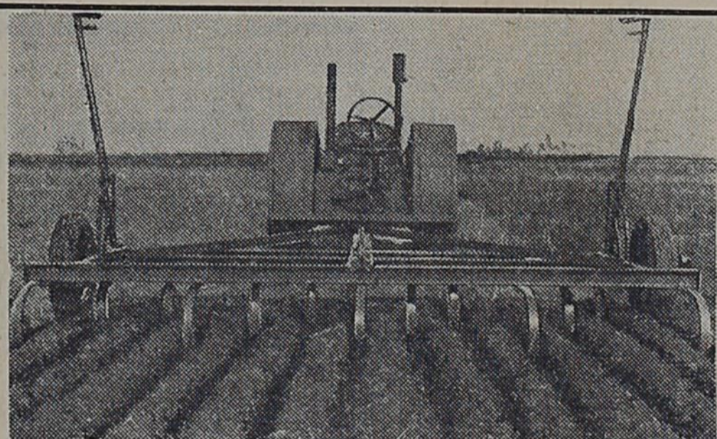
THE JEFFROY "SOIL CONTROL CULTIVATOR"
