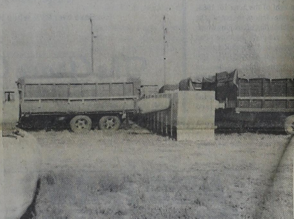
A HANDY CONTRAPTION is this onion dryer used in the on-going onion harvest in the Munday area. The trucks are connected to the dryer which blows hot air into the trucks to dry the onions. It would be difficult to imagine how many onions have been dried by this machine in the last few days, as Munday is in the thick of vegetable harvest.
