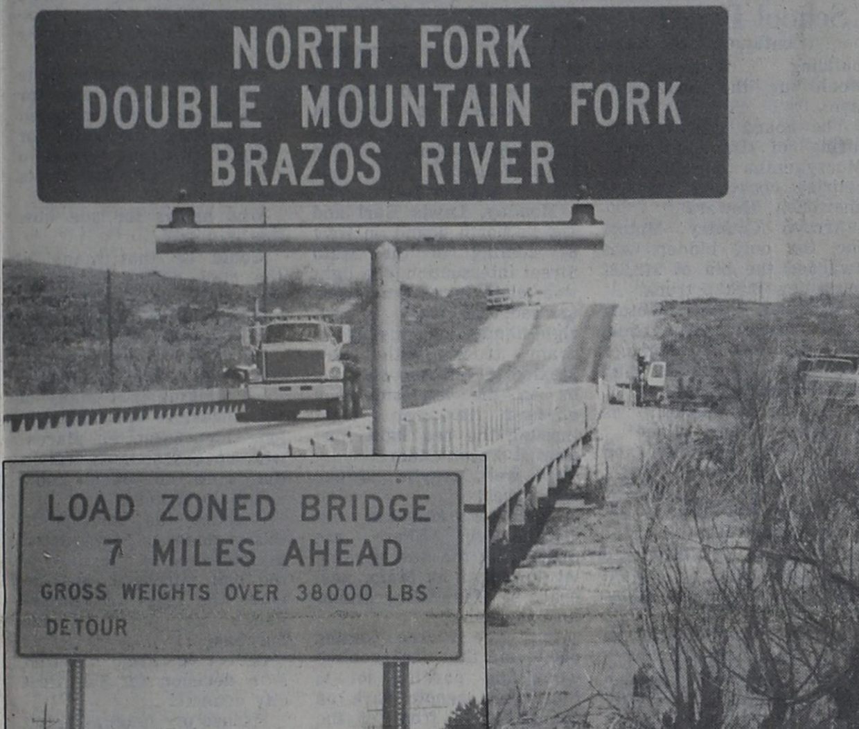
BRIDGE WORK BEGINS - Texas Department of Highways and Transportation crews went to work Monday on adding strength to the bridge crossing U.S. Hwy 380 approximately six miles east of Post. The bridge had been downgraded from 80,000 pounds load to 38,000 pounds, putting a crunch to oil-field and heavy truck traffic east and west bound.
