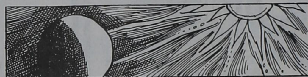
At times during the orbital motion of Uranus, the north or south pole is aligned nearly face on toward the Sun. During those times, the poleward hemisphere receives nearly constant sunlight, while the other hemisphere languishes in decades-long darkness.
