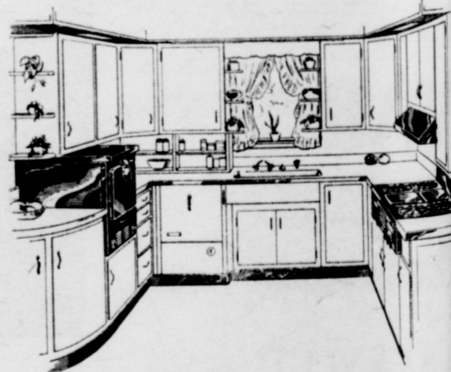
Illustrated above is the Chambers built-in Gas range. This range is approved by the American Gas Association Testing Laboratories.
