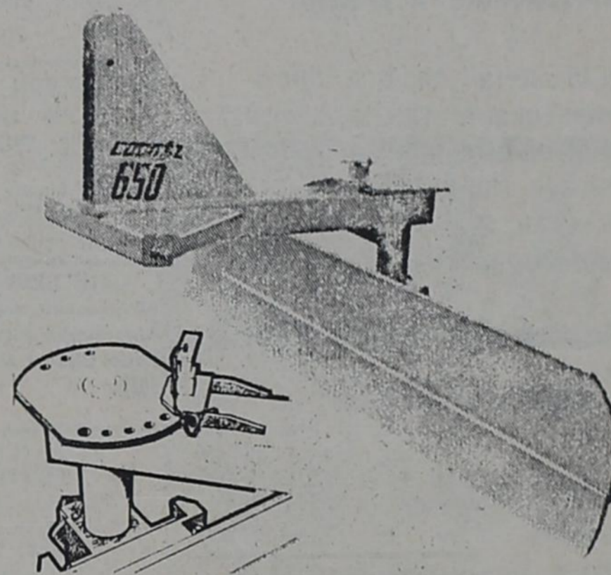
Precision angle adjustment changes angles up to 45 degrees either direction. Locks firmly into place with clevis-type locking pin.
