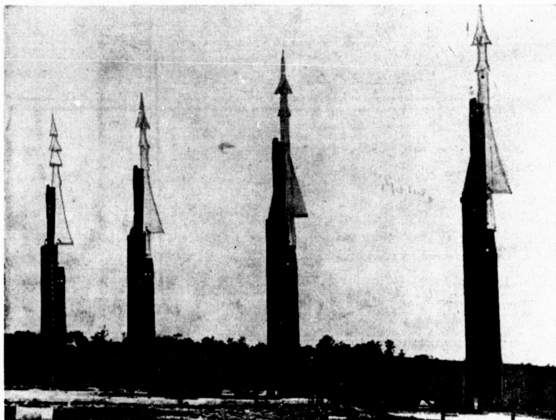
NIKES DEFEND CAPITAL . . . U. S. army's Nike anti-aircraft guided missile station at Lorton, Va., is one of 16 Nike bases ringling Washington. Missiles, shown in firing position, attain speed of 1,500 mph.
