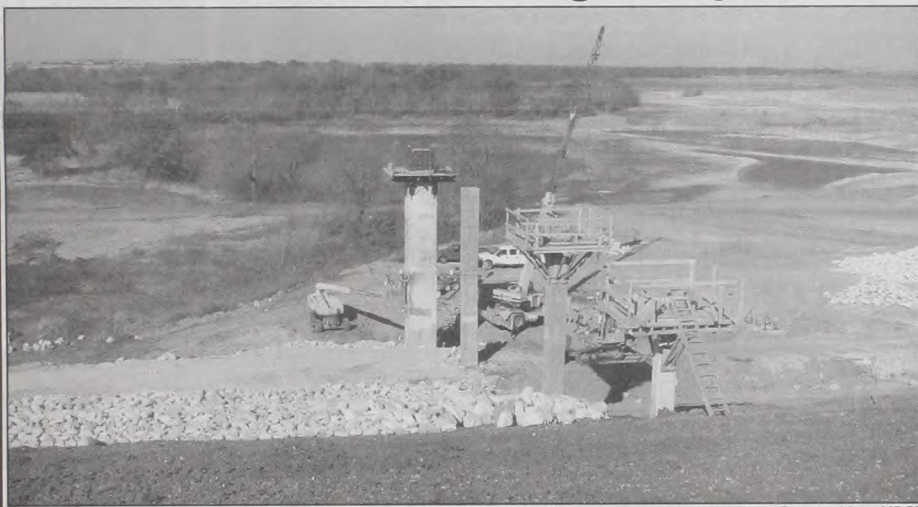
Dam construction at the Muenster Lake project is complete except for a little fill-in and vegetation, according to Raymond Lee, NRCS inspector, who also noted that the spillway is still under construction, but functional. Over 1,350,000 yards of dirt was used to build the dam. Pictured above, work continues on the gate valves that will draw water for the City at three different levels, as the last of the 19,000 tons of rock-rip-rap gets laid to protect the front sloop. In the background is the 308 acres that will one day be under water. Janie Hartman photo
