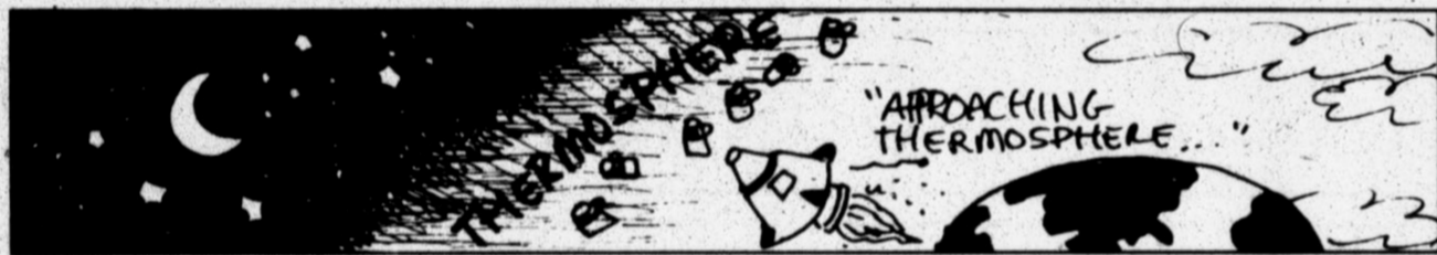
The uppermost region of the earth's atmosphere, beginning at about 50 miles up and continuing into space, is called the thermosphere.
