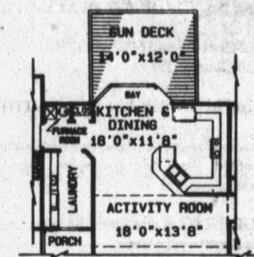
ALT. PART SLAB FLOOR PLAN FOR CRSP OR SLAB FOUNDATION (OMITTING BASEMENT STAIRS)
