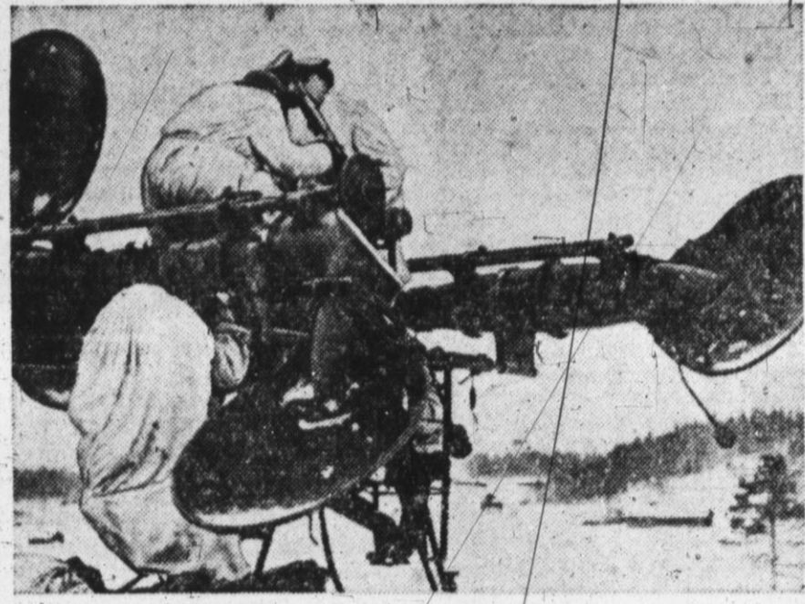
Advance indication of raiding Russian airplanes is given by these sound detectors in the Rovaniemi section of Finland. The "ears" tell the anti-aircraft gunners that planes are approaching before they come into sight.
