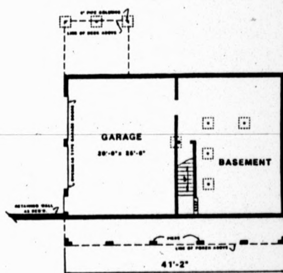
FOUNDATION PLAN
