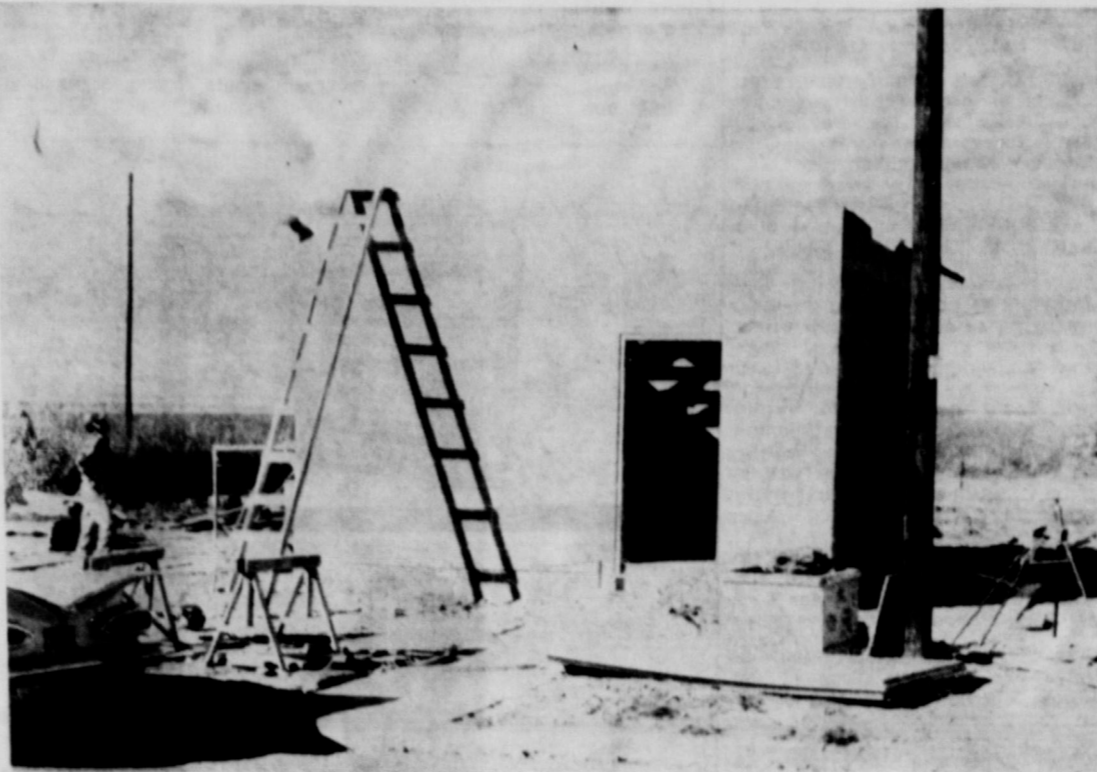
THE NEW SPRINGLAKE TELEPHONE EXCHANGE BUILDING — The 25'x50' building is being erected in Springlake by General Telephone Co. and will house the communication system for the Springlake area. Commercial Contracting Co. is in charge of construction. The building will be near completion by the end of this week.
