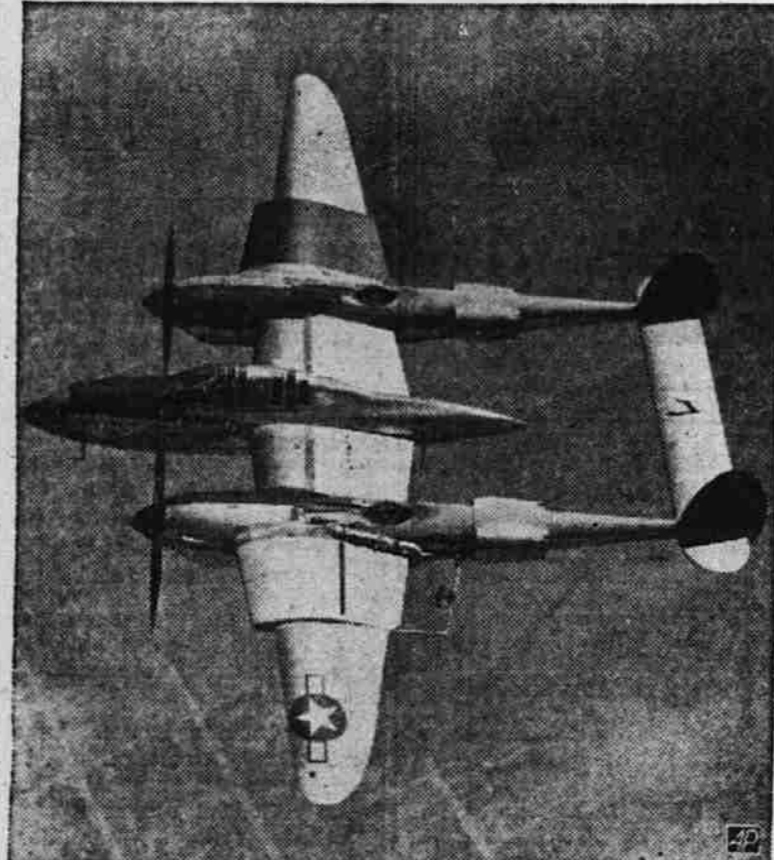
FLYING WIND TUNNEL —This is the Lightning Swordfish, experimental modification of the standard Lockheed P-38 fighter, secretly used to test wing designs of super-fighters and transports since 1943. It is fitted to test drag, lift and airflow characteristics on any type airfoil under actual flying conditions, and dives at more than 525 miles an hour.
