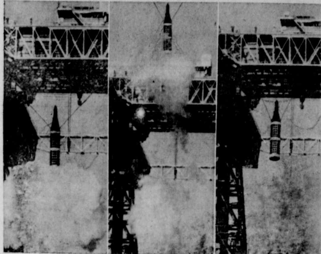
Polaris, deadly ballistic missile designed for firing from submarines, goes through almost-real tests at San Francisco Naval Shipyard. Fully instrumented, it is launched, left. At center, it is snared by arresting gear. At right, it hangs in its spiderweb of lines, ready for lowering and quick check of instruments. This speeds gathering of data over "live" tests.
