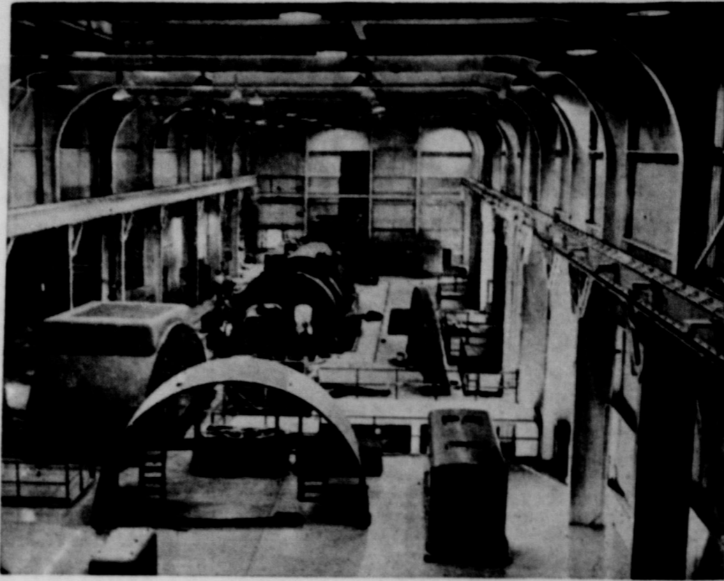
LARGEST UNIT: Pictured under construction at Southwestern Public Service Co.'s Plant X, in Lamb County, Texas, is a 210,000-kilowatt generator. The largest unit ever installed on the company's system, the huge turbo-generator will go into service in mid-
