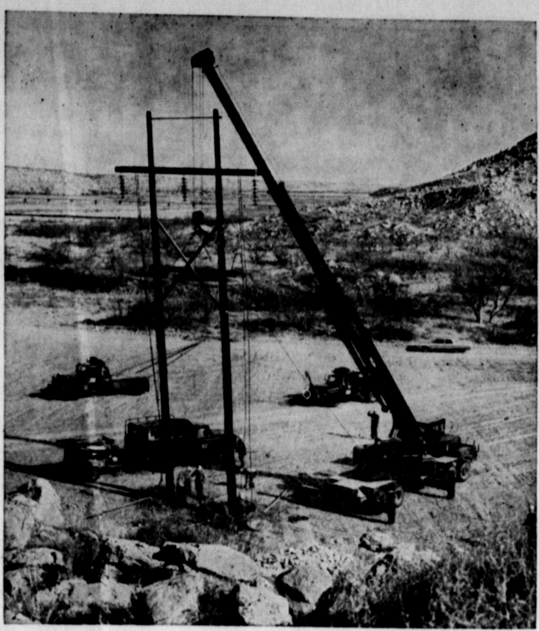
An 80 foot electric transmission line structure can be lifted and set in place in 8½ minutes with Southwestern Public Service Company's new hydraulic crane. The unit, the second one to go into service in the nation, was specifically designed for use in the electric utility industry. Southwestern Public Service Co. has announced a 1966 construction program calling for the investment of $19,353,000 in new facilities, with a large portion of the additional investment to be in transmission lines.
