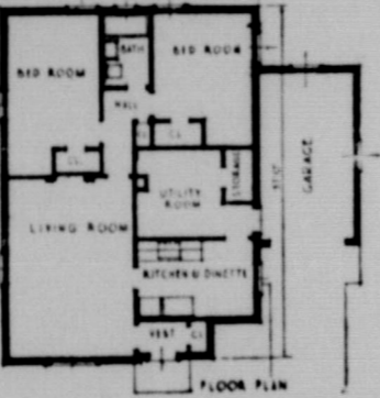
The dwelling shown above is situated in Whitefish Bay, Wisconsin. It is priced at $4,175 and contains five rooms, bath, and an attached one-car garage.
