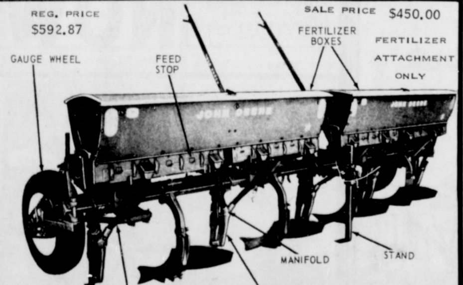
John Deere 275 Fertilizer Attachment on F871 Four-Row Bedder
