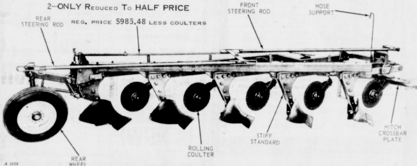
John Deere F135H Five-Bottom Semi-Integral Moldboard Plow with Rippled-Edge Rolling Coulters (Special Equipment)
