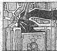
VALVE-IN-HEAD DESIGN
