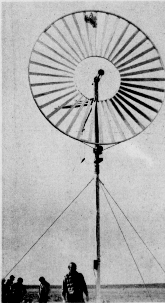
FUTURE ENERGY SOURCE?... When the 'bugs' are worked out, the Muleshoe National Wildlife Refuge has three of these energy generating windmills. They have been installed on a test basis at the refuge. The mill shown here operates the electric pump in the background. Facing the camera is Al Jones, refuge manager.
