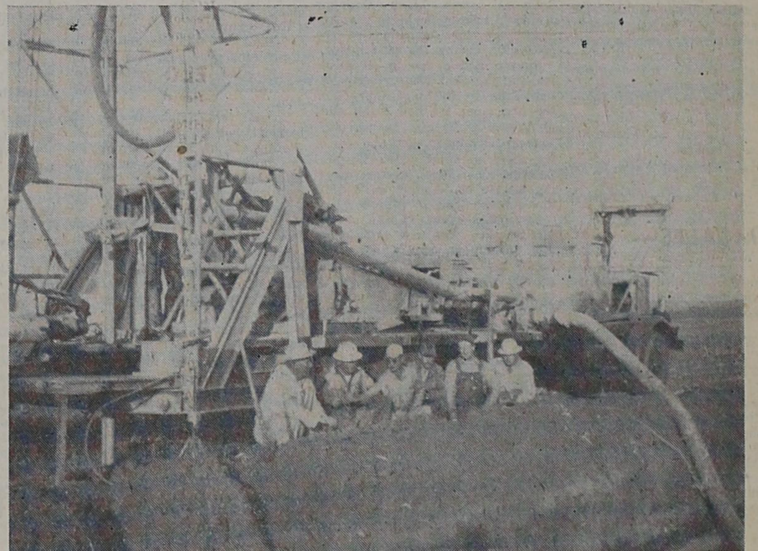
The above picture gives a small idea of the size of this oilfield-type rotary drilling rig, which weighs over 55,000 pounds. It is one of the biggest and best equipped rigs available for drilling irrigation wells anywhere.
