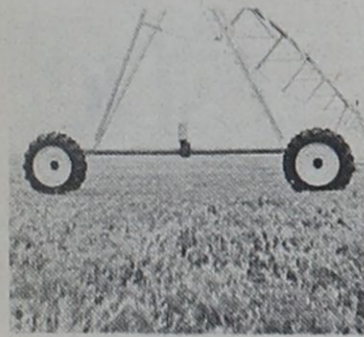
Extra Long Wheelbase: A full 14 ft. - one of the longest in the industry. Works with Uni-Knuckle and Lindsay rolling feature to provide exceptional stability on rough terrain and over terraces.
